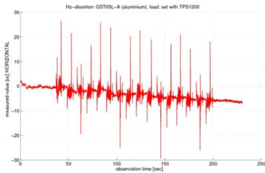
Figure 6b - trépied Leica GST05L
