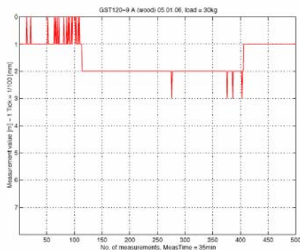
Figure 3a - trépied Leica GST120-9
