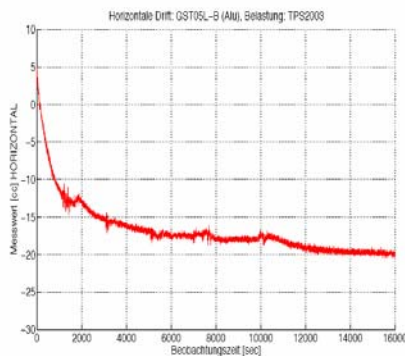
Figure 8b - trépied Leica GST05L
