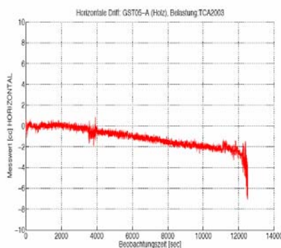
Figure 8c - trépied Leica GST05
