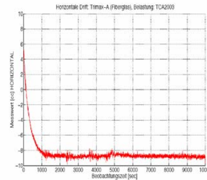
Figure 7c - trépied Crain Trimax
