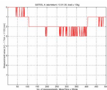
Figure 4b - trépied Leica GST05L
