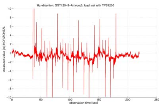
Figure 5a - trépied Leica GST120-9
