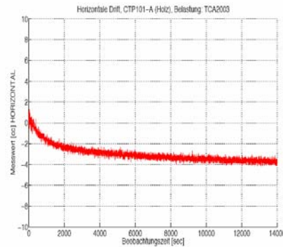
Figure 7b - trépied Leica CTP101
